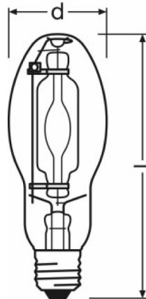
HQI-E 70 W/NDL CL, HQI-E 100 W/NDL CL, HQL-E 150 W/NDL CL
